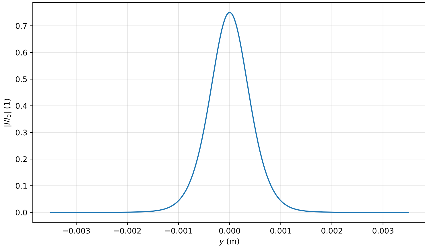
Intensity profile I(x=0, y, z=2.707)/I_0 , P_{in}=0.6P_{cr} , artificial time
